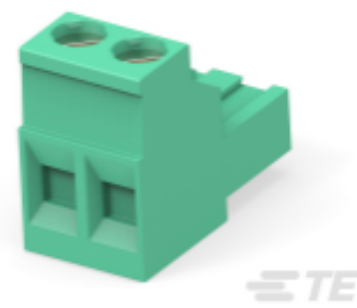
TE Part # 796640-2 2 POS 5.0 MM R/A PLUG, TRM BLK
